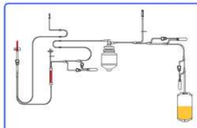
P-1000H 带取全血样试管、盐水补偿和两个血浆留样试管
